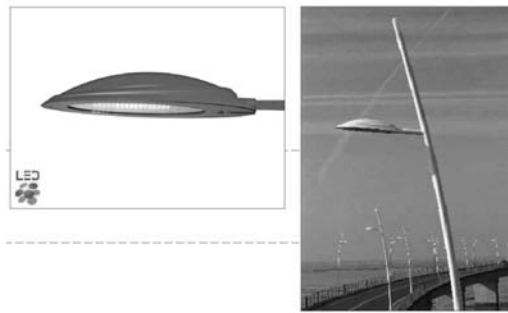
LED STREET LIGHT MFR: LUMEC MODEL: CAPELLA LED COLOR: SILVER ALUMINUM POLE: HAPCO #B32079 COLOR: SILVER
