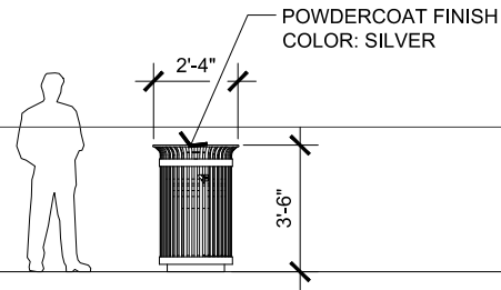
TRASH/RECYCLING RECEPTACLES VICTOR STANLEY SD-42 CONVEX AND RECYCLE LID SURFACE MOUNT WITH LOCK
