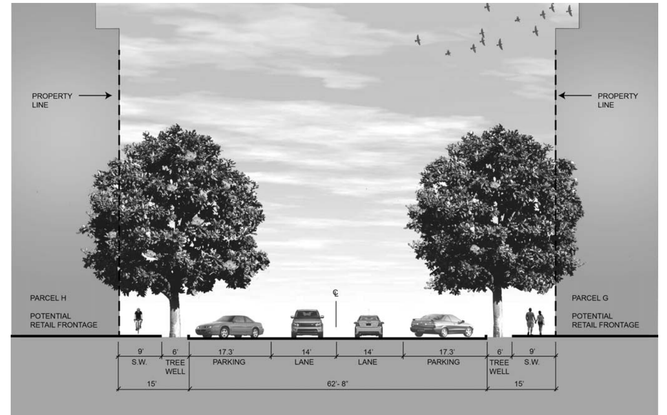
SECTION 2 - MAIN STREET
