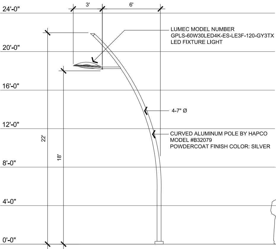
PHASE I ONSITE LED STREET LIGHT LUMEC CAPELLA LED LIGHT DISTRIBUTION IES TYPE 3 BUG RATING - B1-U0-G1
