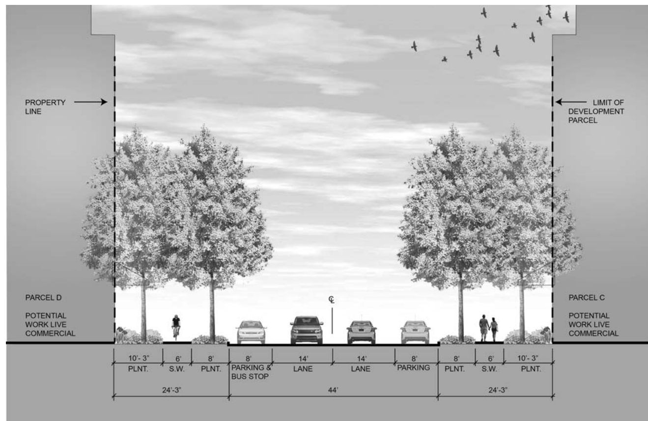
SECTION 3 - MAIN STREET
