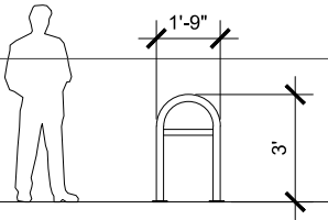
BIKE RACK THE PALMER GROUP WELLE SERIES EMBEDDED GALVANIZED ADA CROSS BAR SU-20-F-SS-CB
